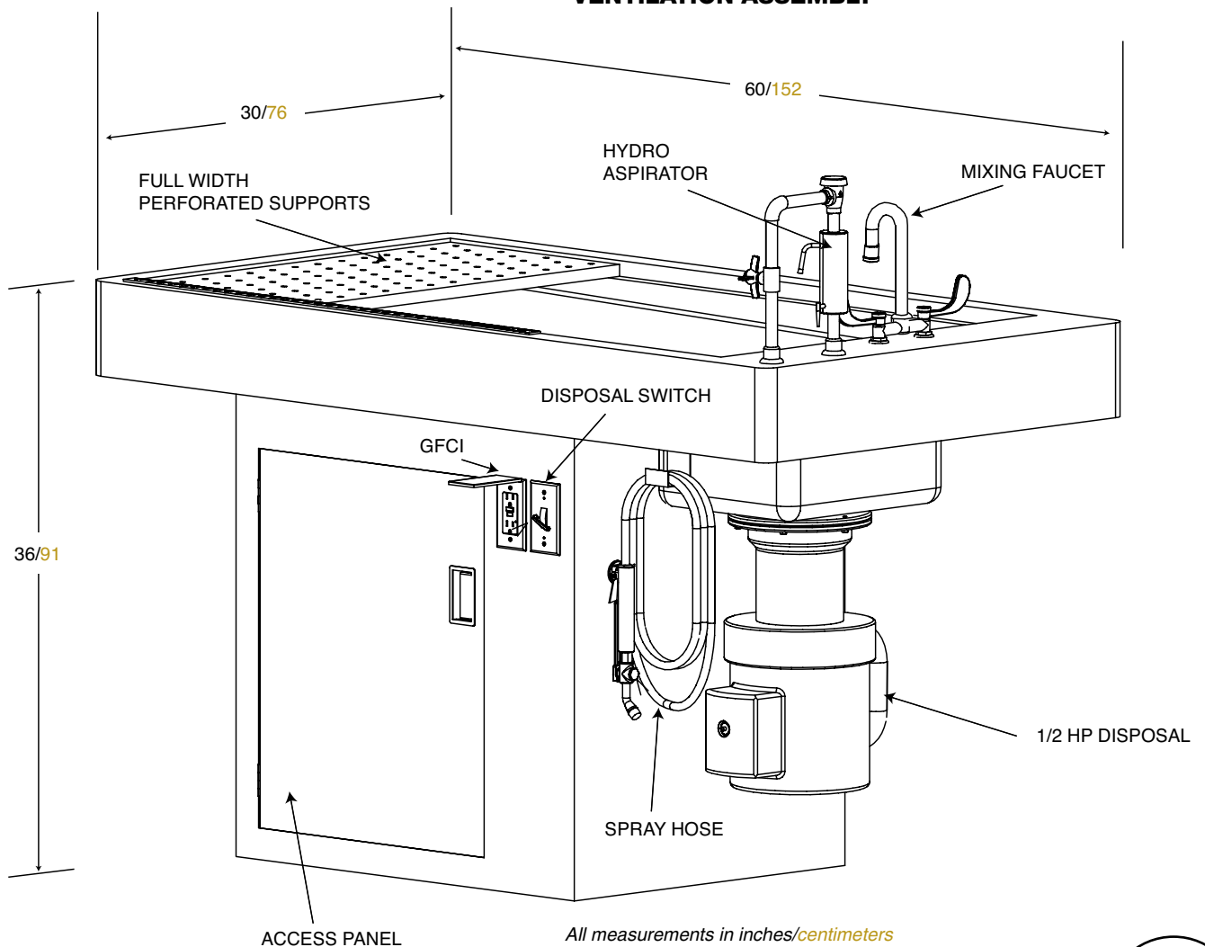
DOUBLE-CONE DOWN DRAFT VENTILATION ASSEMBLY
