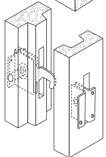
CAM-LOC FASTENERS
