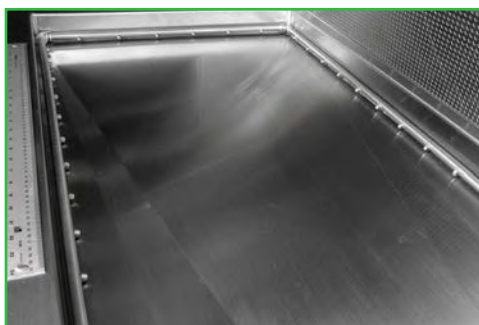
OA-301 - THREE SIDED RINSE ASSEMBLY Provides a rinse to gently wash debris and non-viable material away from the work area. A sturdy stainless steel assembly controlled by an on/off valve.
