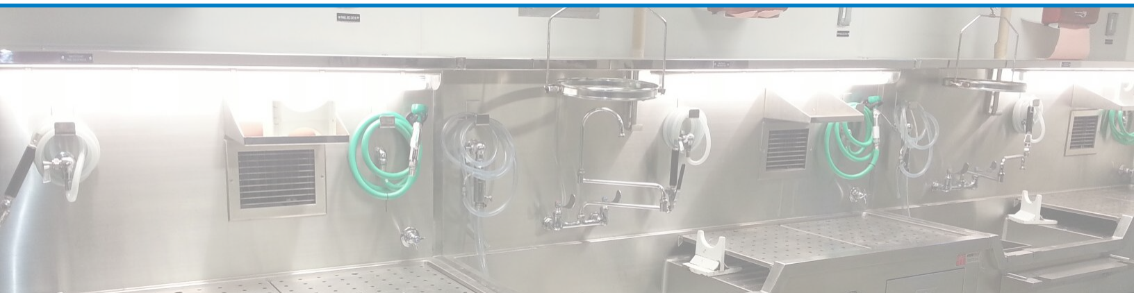
OA-201 - FORMALIN DISPENSING AND COLLECTION 2.5 gal. container and receptacle hold reserve formalin and collects waste. Foot controlled motor dispenses formalin at a steady flow. Conveniently placed formalin supply spout included.
